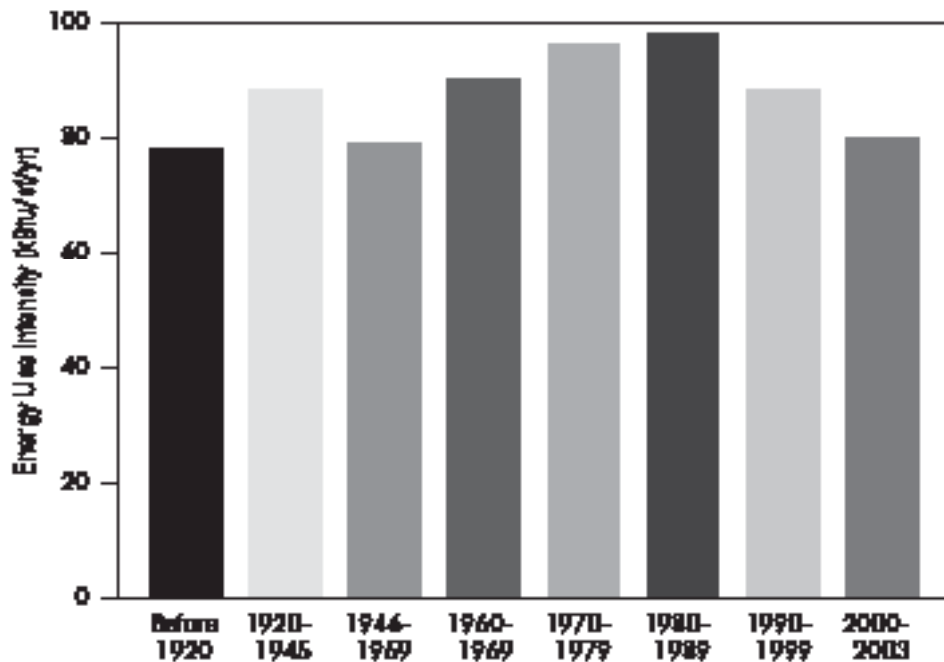
FIGURE 3 Actual Measured Energy Consumption versus Year Constructed for Canadian Commercial Buildings
