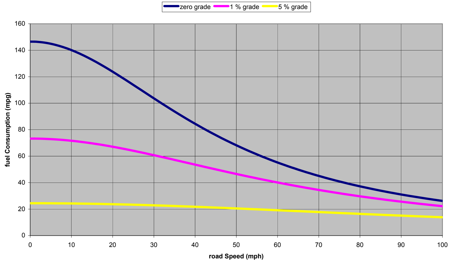
Prius Fuel Consumption with Grade
